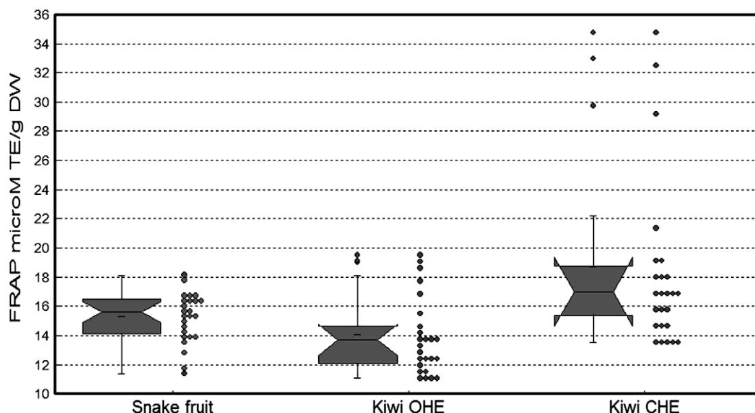
Fig. 4. Box and dot plots of the frequency distribution of the snake fruit, and two kiwifruit samples: conventional 'Hayward' (CHE) and organic 'Hayward' ethylene treated.
