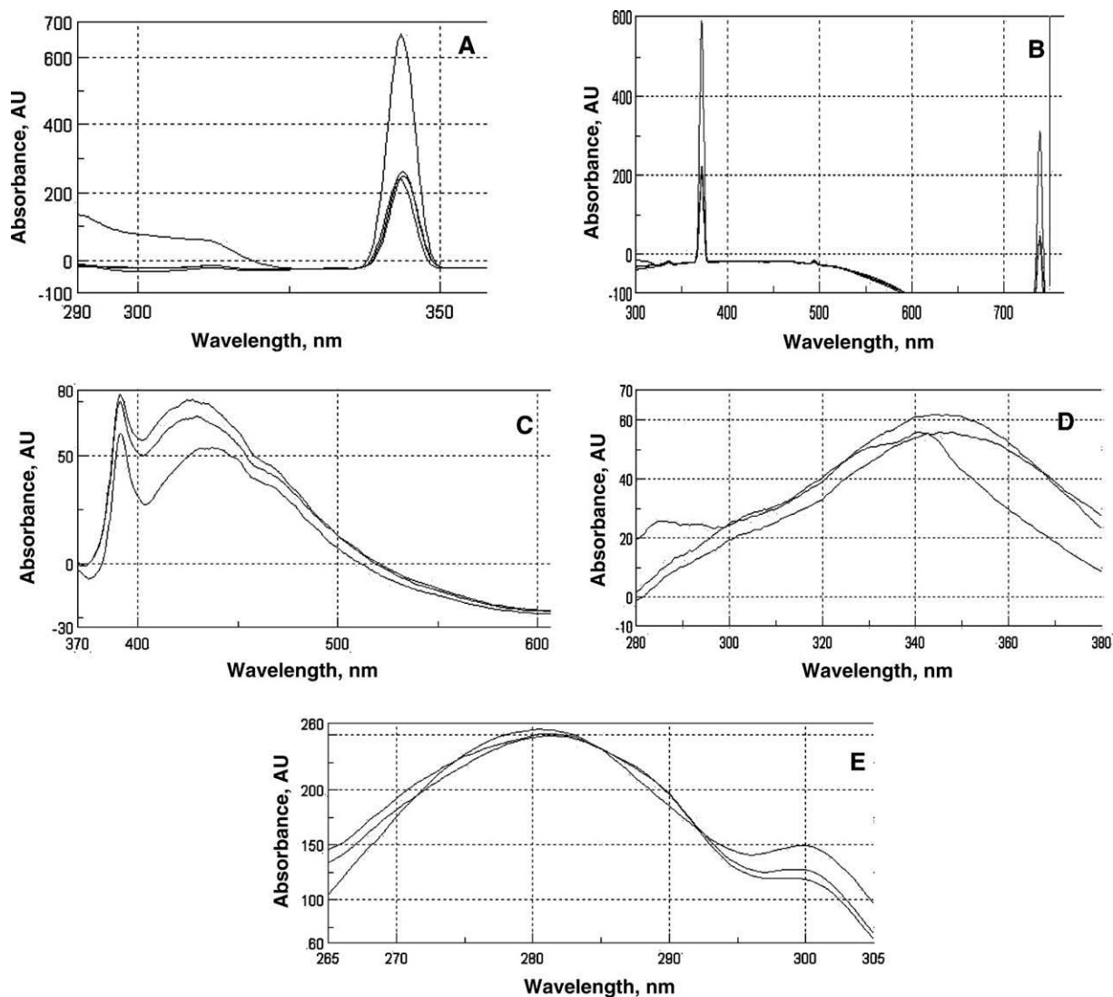
Fig. 2. Fluorimetric excitation spectra of fruit extracts (0.25 mg/ml) with: (A) emission wavelength at: 685 nm recorded over the frequency range from the excitation wavelength from 290 to a wavelength of 400 nm from upper to lower lines: catechin, organic and conventional kiwifruit, snake fruit; (B) emission at 740 nm and recording from 300 to 750 nm; (C) excitation at 350 nm and recording from 370 to 650 nm; (D) emission at 450 nm and recording from 280 to 380 nm; (E) emission at 330 nm and the recording from 265 to 305 nm.
