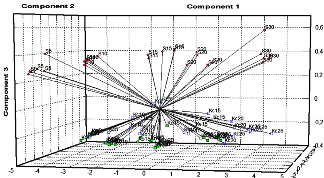
Fig. 3. Principal component analysis of FRAP parameters of snake fruit (S), Kiwi OHE (Ko) and kiwi CHE (Kc) extracts (5–25 mg/ml).
