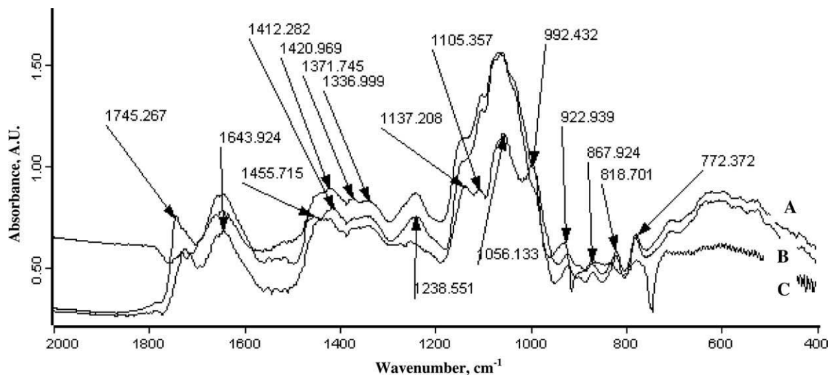
Fig. 1. FT-IR spectra of shake fruit (line C), organic (line A) and conventional (line B) kiwifruit.
