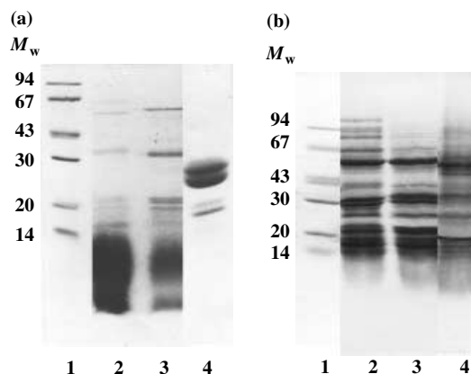
Figure 1 Sodium dodecyl sulphate polyacrylamide gel electrophoresis in 5–20% polyacrylamide gel of total alcohol-soluble proteins (TASP) in (a) lane 1, molecular marker (94, phosphorylase b; 67, haemoglobin, canine; 43, ovalbumin; 30, carbonic anhydrase; 20, trypsin inhibitor, soybean and 14, lactalbumin, bovine milk); lane 2, amaranth; lane 3, soybean; lane 4, maize; of total buffer-soluble proteins- total glutelins (TGlu) in (b) lane 1, the same molecular marker as in (a); lane 2, amaranth; lane 3, soybean; lane 4, maize. TASP were extracted with 55% (v/v) isopropanol (IP), containing 4% (v/v) 2-mercaptoethanol (2-ME); TGlu with 0.125 M sodium borate buffer, pH 10, containing 3% (v/v) 2-ME and 1% sodium dodecyl sulphate (SDS) (w/v).
