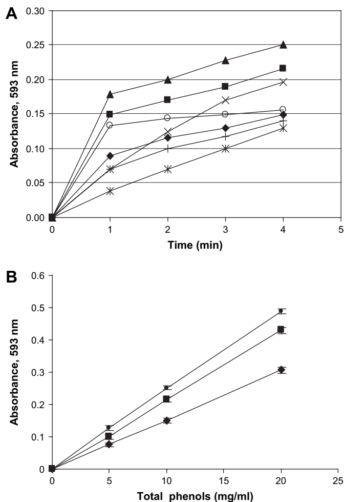
Fig. 3. FRAP (Ferric-reducing/antioxidant power) measurements of durian extracts with two variables (different concentrations and different periods of time): A, total polyphenol extracts of durian cultivar Mon Thong at different stages of ripening: (◆) M, mature; (■) O, overripe; (▲) R, ripe at constant concentration (10 mg/ml) and with the change of time (1, 2, 3, and 4 min). Standards (30 \mu\text{g/ml} ), (×) NAR, (*) FIC, (+) QUER, naringin, ficitin and quercetin, respectively; (○) GA, gallic acid, 10 \mu\text{g/ml} ; B, total polyphenol extracts from durian cultivar Mon Thong at different stages of ripening: (◆) C, mature; (■) D, overripe; (●) G, ripe at constant time (4 min) with the change of extracts concentration (5, 10, 15 and 20 mg/ml).
