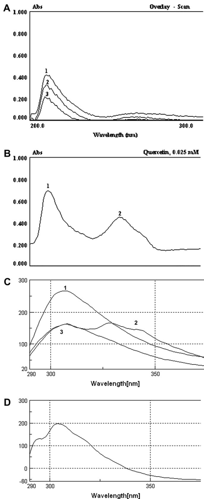
Fig. 1. UV absorption spectra of methanol extracts recorded from 195 to 400 nm. A, free polyphenols (0.02 mg/ml) of ripe (1), overripe (2) and mature (3) durian fruit. B, quercetin (0.025 mM). Fluorimetric spectra of methanol extracts taken at excitation wavelengths (nm) of 270 and emission of 290 recorded over the frequency range from the excitation wavelength to a wavelength of 500 nm. C, free polyphenols (0.02 mg/ml) of ripe (1), overripe (2) and mature (3) durian fruit. D, quercetin (0.01 mM).
