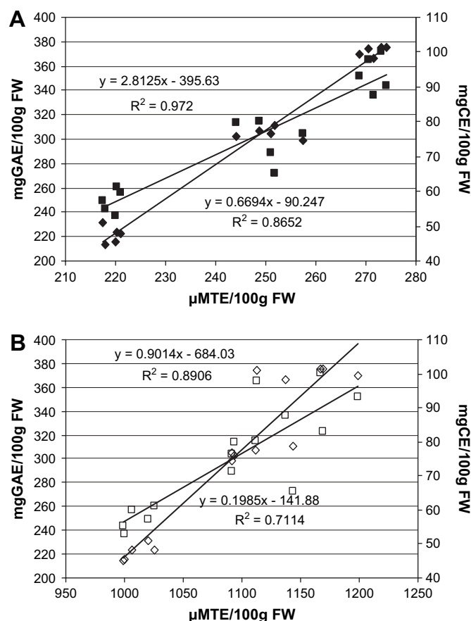
Fig. 4. Correlation between measures of antioxidant capacities (AC) and total phenolics (TPOL). A, (◆) ACFRAP ( \mu\text{MTE}/100\text{ g FW} , X) and TPOL (mg GAE/100 g, Y_1 ), (■) ACFRAP ( \mu\text{MTE}/100\text{ g} , X) and TFLAV (mg CE/100 g FW, Y_2 ). B, (◇) ACCUPRAC ( \mu\text{MTE}/100\text{ g} , X) and TPOL (mg GAE/100 g, Y_1 ), (□) ACCUPRAC ( \mu\text{MTE}/100\text{ g} , X) and TFLAV (mg CE/100 g, Y_2 ). Abbreviations: FRAP, Ferric-reducing/antioxidant power; CUPRAC, Cupric-reducing antioxidant capacity; TPOL, Total polyphenols; TFLAV, Total flavonoids.
