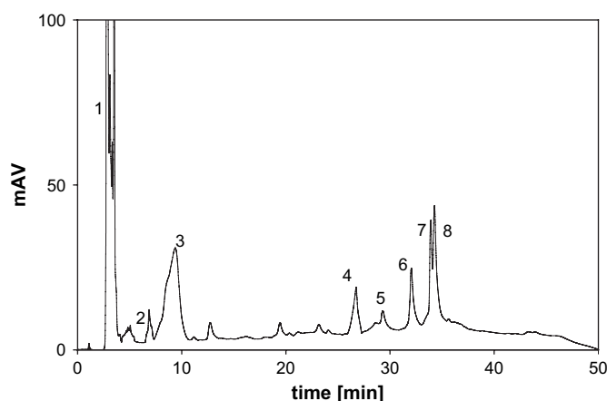
Fig. 2. The chromatogram obtained from the Durian overripe extract. The identified compounds: (1) vanillic acid; (2) caffeic acid; (3) cinnamic acid; (4) morin; (5) neohesperdigo; (6) myricitin; (7) apigenin; and (8) campherol.
