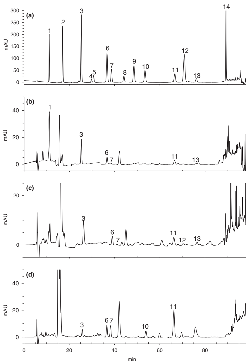
Figure 3 HPLC analysis of methanol soluble ester-bound phenolic acids extracted from fruits. Each profile represents an equivalent amount of extract, normalised on a volume of extract per 5 mg of tissue basis. Chromatograms are showing the separation: a, standard mixture; b, Mango; c, Avocado; d, Durian. 1, gallic acid; 2, protocatechuic acid; 3, p -hydroxybenzoic acid; 4, m -hydroxybenzoic acid; 5, 2,3 dihydroxybenzoic acid; 6, vanillic acid; 7, caffeic acid; 8, chlorogenic acid; 9, syringic acid; 10, p -coumaric acid; 11, ferulic acid; 12, anisic acid; 13, sinapic acid; 14, cinnamic acid.
