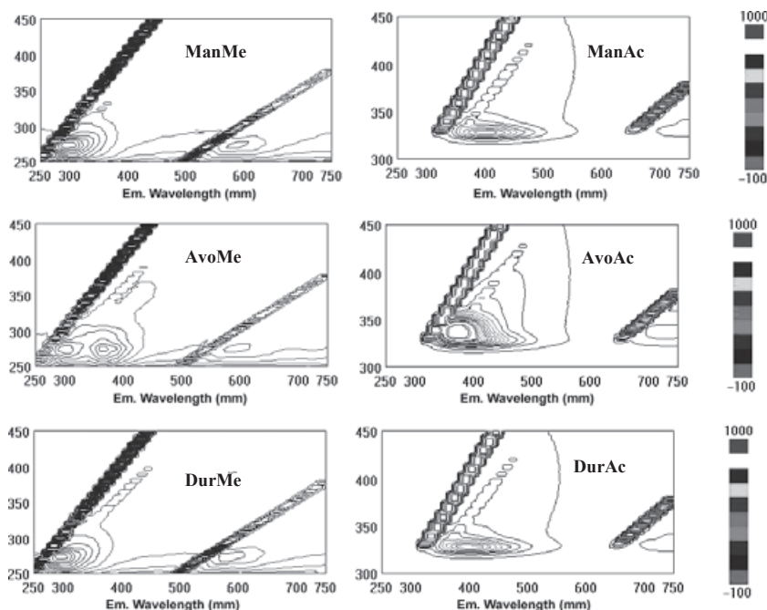
Figure 2 The contour map of methanol (Me) and acetone (Ac) extracts of mango (Man), avocado (Avo), durian (Dur), respectively, displayed a view of the corresponding three-dimensional fluorescence spectra (3-D FL). Fluorescence intensity values from < 100 to 1000 are presented. Details of the experiment are presented in Materials and Methods and in Supporting Information.
