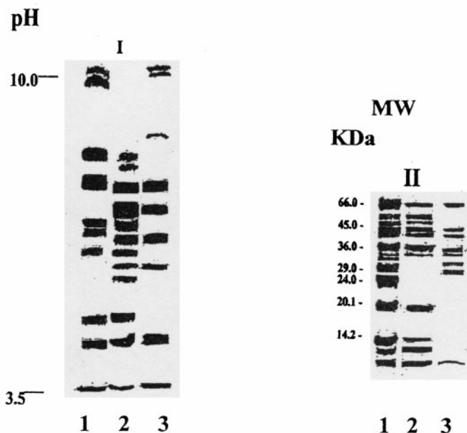
Fig. 2. Electrophoretic analyses of beer and white wine proteins. I – electrofocusing: lane 1, molecular marker; lane 2, 3 – proteins precipitated with acetone from beer and white wine. M_{Ip} markers had the following pH range: 3.5–10. II – SDS-PAGE separation on homemade mini gradient gels of 10–20%: lane 1 –molecular marker; lanes 2,3 - proteins precipitated with acetone from beer and white wine. M_w markers had the following sizes: 14.2; 20.1; 24; 29; 36; 45 and 66 kDa.
