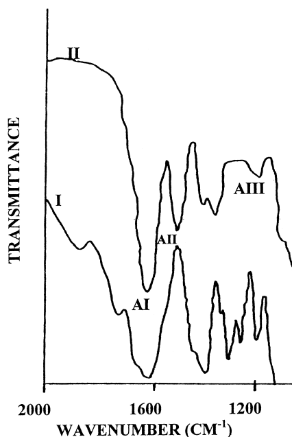
Fig. 3. FT-IR spectra of proteins from: (II), beer; (I), wine. A I, A II and A III - amide I, II and III bands, respectively.
