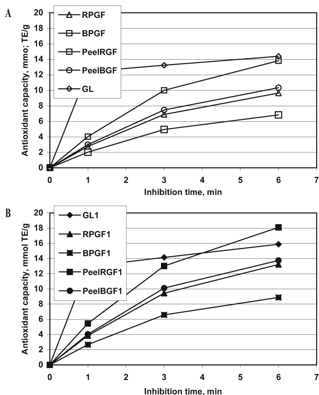
Fig. 2 Kinetics of 2,2'-azinobis(3-ethyl-benzothiazoline-6-sulfonic acid) diammonium salt (ABTS) scavenging effect of citrus extracts. The concentration of the samples was 0.25 mg/ml. a ABTS was produced by reacting potassium persulfate with RPGF, BPGF, PeelRGF and PeelBGF; GL, glutathione. b ABTS + radical cation was produced by reacting manganese dioxide with red peeled grapefruit (RPGF1), blond peeled grapefruit (BPGF1), peels of red grapefruit (PeelRGF1) and peels of blond grapefruit (PeelBGF1); GL1, glutathione.
