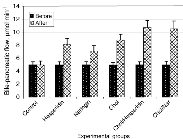
Figure 2. Changes in the pancreatic–bile flow ( n = 10 ). Addition of hesperidin and naringin significantly increased the pancreatic–bile flow ( P < 0.05 ).
