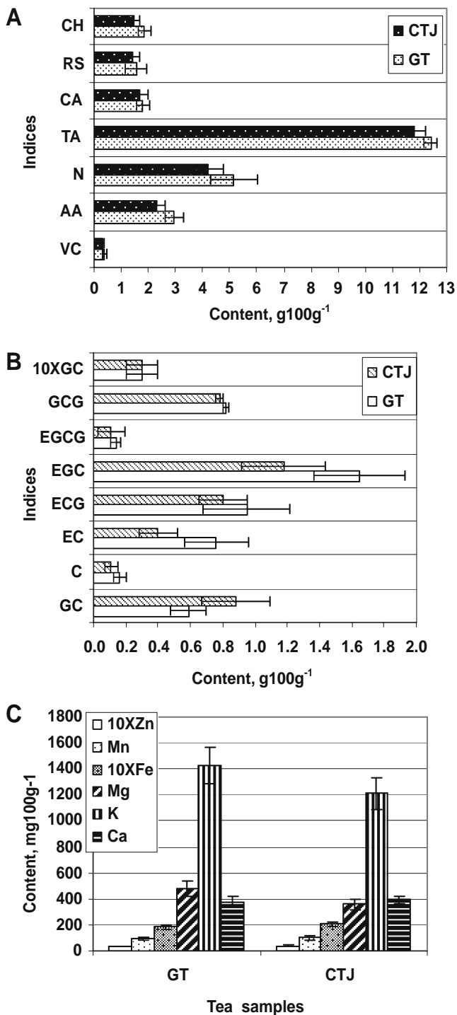
Fig. 3 Partial characterization of Chungtaejeon tea (CTJ) and green tea (GT). A , Indices of Vitamin C (VC), Reducing sugars (RS), Caffeine (CA), Tannin (TA), Total nitrogen (N), Total amino acids (AA), Chlorophyll (CH); B , Contents of catechins in Chungtaejeon and green tea: 10XGallocatechin (10XGC), Gallocatechin gallate (GCG), Epigallocatechin gallate (EGCG), Epigallocatechin (EGC), Epicatechin (EC), Catechin (C), Epicatechin gallate (ECG), Catechin gallate (CG); C , Contents of minerals
