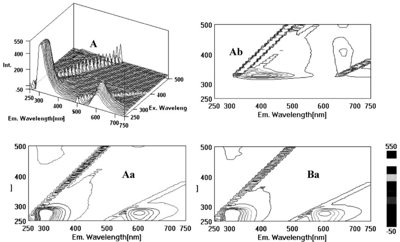
Fig. 1 Three dimensional fluorescence map of 0.005 mg/mL of methanol extracts of Chungtaejeon tea (CTJ, A). The contour maps (Aa and Ba) displayed a view of the corresponding fluorescence spectra of 0.005 mg/mL of methanol extracts of CTJ and green teas; and (Ab) of 0.02 mg/mL of acetone extracts of Chungtaejeon
