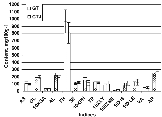
Fig. 4 Amino acid content in Chungtaejeon and green tea, teas. AS, Aspartic acid; GL, Glutamic acid; 10XGA, Gaba; AL, Alanine; TH, Threonine; SE, Serine; 10XPH, Phenylalanine; 10XPH, Phenylalanine; TR, Tryptophan; 10XLY, Lysine; 100XME, Methionine; 10XIS, Isoleucine; 10XLE, Leucine; VA, Valine; AR, Arginine
