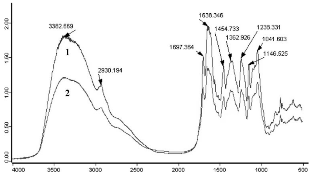
Fig. 2 FTIR spectra of Chungtaejeon (1) and green (2) tea samples
