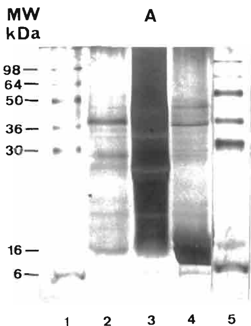
Fig. 2. Electrophoretic separation of cactus proteins (peak B in Fig. 1) in SDS-gradient gel 10–15% PAAG. Molecular weight marker (lane 1), Pitahaya agria (lane 2), Garambullo (lane 3), Cholla (lane 4), molecular weight marker (lane 5). Proteins were detected by silver staining.
