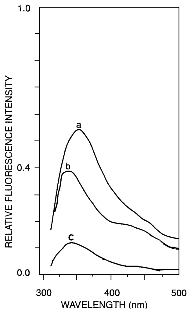
Fig. 4. Fluorescence emission spectra of proteins from Pitahaya agria (a), Garambullo (b), and Cholla (c). Excitation at 295 nm.
