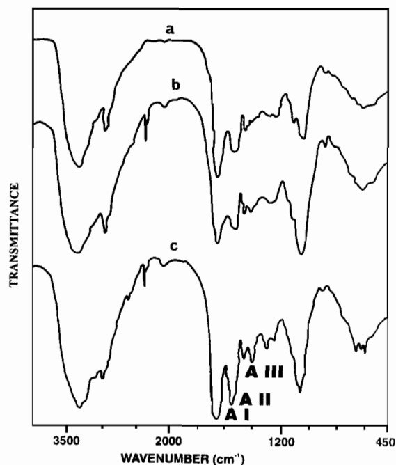
Fig. 5. FT-IR spectra of proteins from Garambullo (a), Pitahaya agria (b), and Cholla (c).
