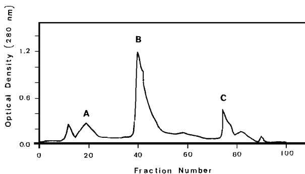
Fig. 1. DEAE-Sepharose chromatographic patterns of crude cactus from Pitahaya agria.
