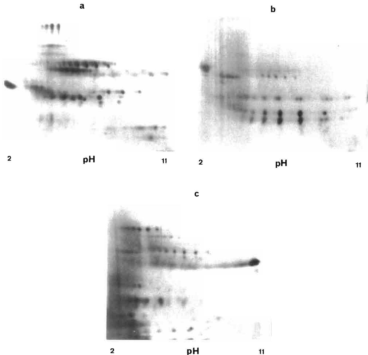
Fig. 3. Electrophoretic separation of cactus proteins (peak B in Fig. 1) in 2DE: (a) Pitahaya agria, (b) Garambullo, (c) Cholla. Samples were applied at the anodic side of the IEF gel. Proteins were detected by silver staining.
