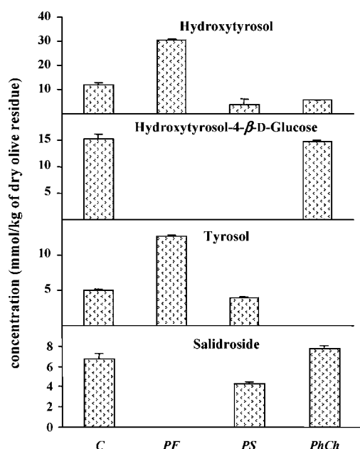
Figure 5. Main monomeric phenols in DOR treated for 2 weeks with Pa. farinosus (PF), Po. subvermispورا (PS), and Pha. chrysosporium (PhCh). Data in untreated DOR have also been included. Error bars are standard deviation ( n = 2 ).
