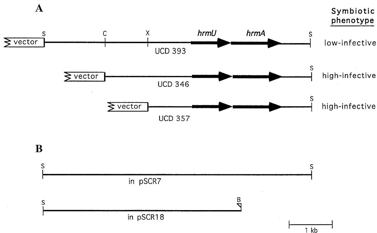
Fig. 2. Aligned maps of hrmUA DNA found in the chromosome of selected Nostoc punctiforme 29133 single recombinant strains and in two multicopy plasmids. A , Effects of truncations in the DNA 5' to the wild-type copy hrmUA sequence on the symbiotic phenotype of single recombinant strains where the initial recombination occurred upstream of the insertion of \Omega - npt (strains UCD 393 [ hrmA ] and 357 [ hrmU ] or luxAB (strain UCD 346 [ hrmU ])). Sequences upstream of the identified vector position contains the interrupted gene copy and various amounts of DNA 3' of the interrupted gene. B , Fragments of Nostoc DNA carried in the multicopy plasmids pSCR7 and pSCR18. Restriction sites are for Bam HI, B (originally from the lux end of Tn5-1063); Cl aI, C; Spe I, S; and Xba I, X.
