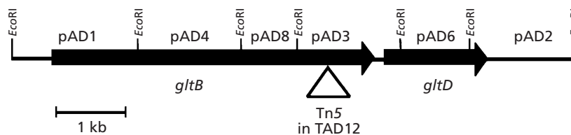
Fig. 1. Physical map of cosmid pC12 harbouring gltB and gltD GOGAT-encoding genes, showing the position of the Tn5 insertion in mutant TAD12.
