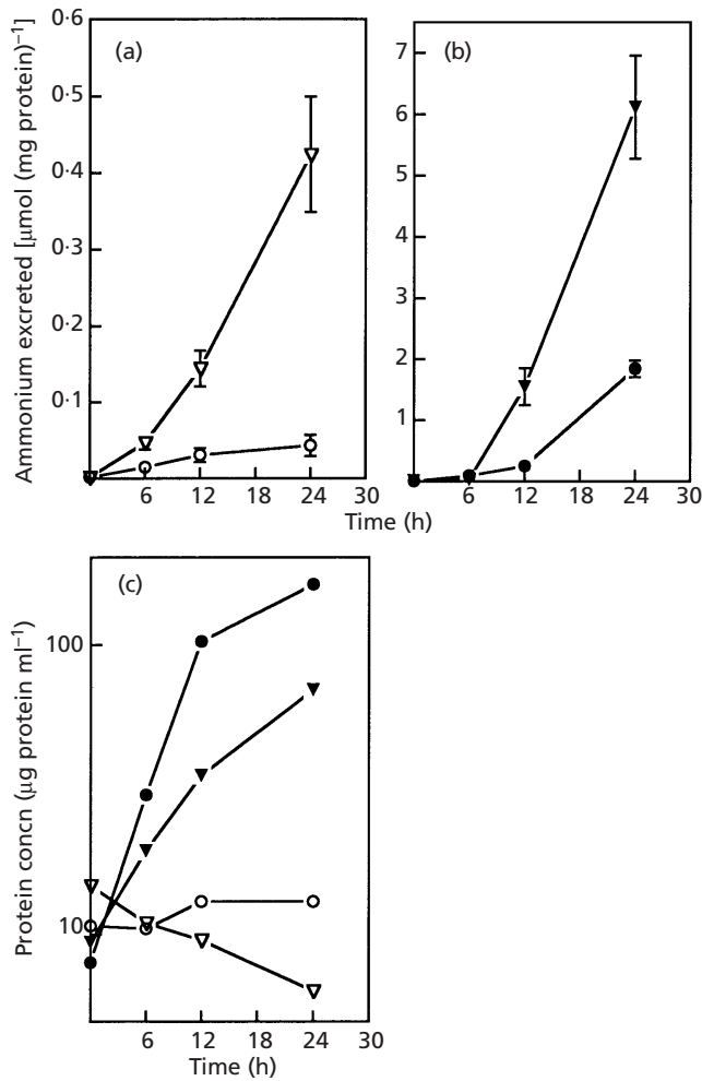
Fig. 3. Ammonium excretion by the CFN42 wild-type and TAD12 mutant strains with and without glutamate. Rhizobium strains were cultured in MM and aliquots were withdrawn at the indicated times to measure extracellular ammonium as indicated in Methods. (a) Ammonium excretion in MM with succinate (30 mM) without nitrogen source; CFN42 wild-type strain (○) and TAD12 mutant (▽). (b) Ammonium excretion in MM with succinate (30 mM) plus glutamate (10 mM) as nitrogen source; CFN42 wild-type strain (●) and TAD12 mutant (▼). The results are from three independent experiments. (c) Protein concentration of the CFN42 wild-type (○) and TAD12 mutant (▽) strains corresponding to culture conditions as in (a), and CFN42 wild-type (●) and TAD12 mutant (▼) strains corresponding to culture conditions as in (b).
