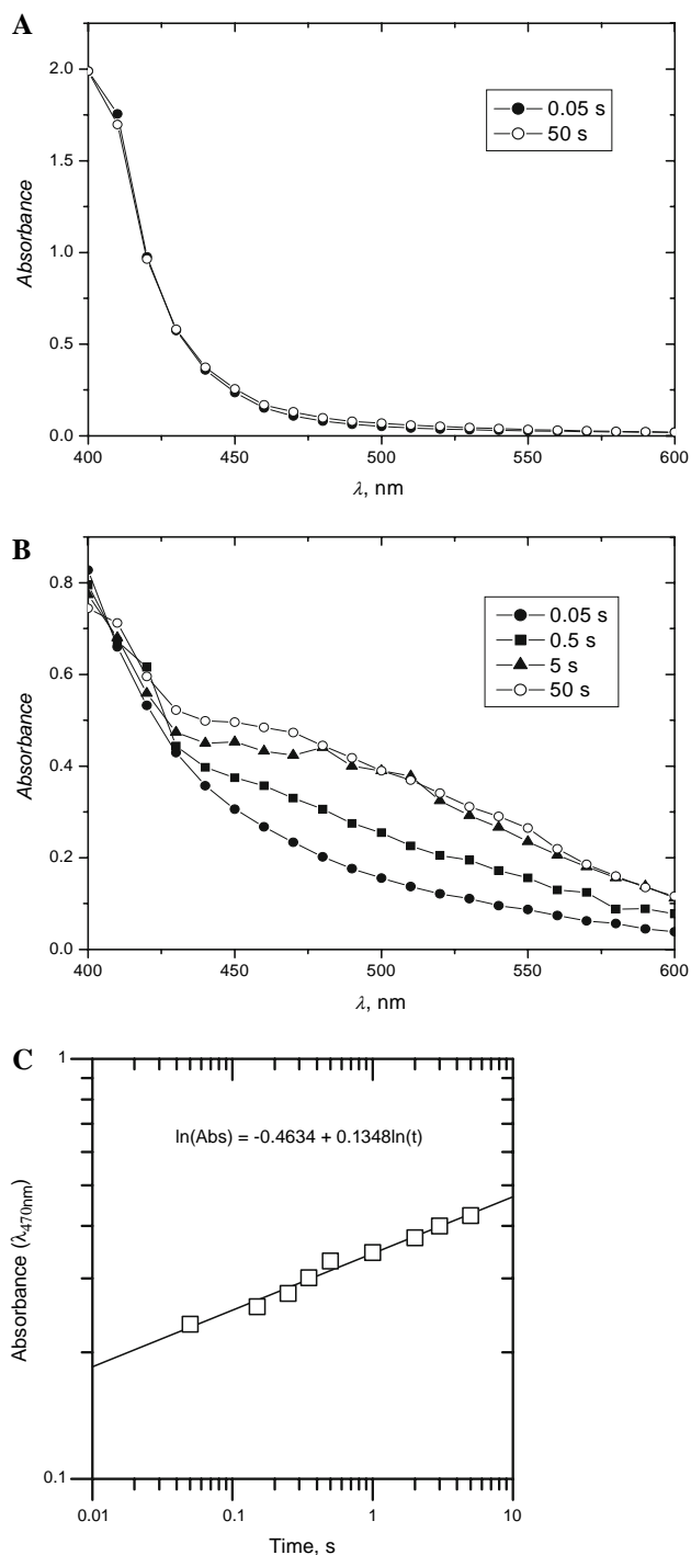
Fig. 1 Rapid scan time course of the reaction of FeCl 3 with IAA at 25°C. (a) molar ratio of 1:3 (Fe III :IAA) in absolute ethanol. (b) molar ratio of 1:12 (Fe III :IAA) in ethanol–water solvent (50:50v/v), (c) increase of the absorbance at \lambda = 470 nm in the ethanol–water mixture (50:50v/v)
