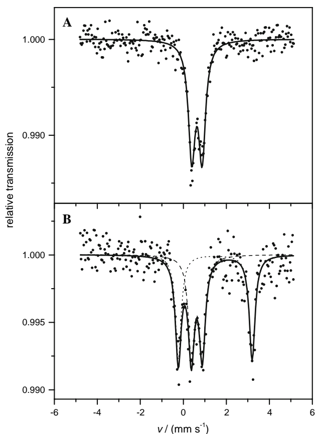
Fig. 7 Mössbauer spectra of the reaction mixture of \text{Fe}(\text{NO}_3)_3 \cdot 9\text{H}_2\text{O} and IAA at a molar ratio of 1:3 ( [\text{Fe}^{3+}] = 0.1 \text{ M} ). Mixtures were prepared in (a) absolute ethanol and (b) in ethanol–water solvent (50:50v/v). Solutions were frozen after 20 min and spectra were taken at 100 K
