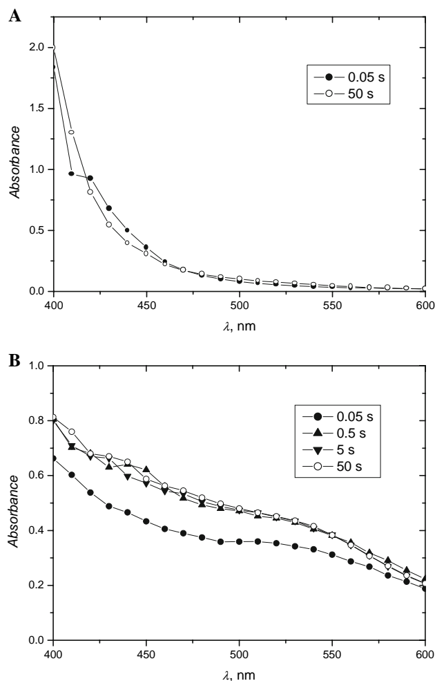
Fig. 2 Rapid scan time course of the reaction of FeCl 3 with IAA at 25°C. (a) molar ratio of 1:3 (Fe III :IAA) in acetone (b) molar ratio of 1:12 (Fe III :IAA) in acetone–water solvent (50:50v/v)
