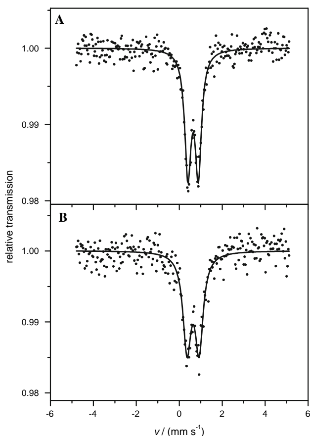
Fig. 6 Mössbauer spectra of the ^{57}\text{Fe} –IAA solid complex redissolved in absolute ethanol (a) and in ethanol–water solvent (50:50v/v) (b). Solutions were frozen after 20 min and spectra were taken at 100 K
