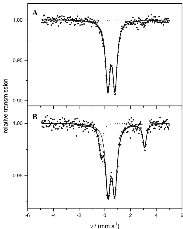
Fig. 5 Mössbauer spectra of the mixture of ^{57}\text{FeCl}_3 and IAA at a molar ratio of 1:3 ( [\text{Fe}^{3+}] = 0.025 \text{ M} ). Reaction mixture was prepared in ethanol–water solvent (50:50v/v) and solution was frozen at (a) 50 s, (b) 20 min. All spectra were recorded at 100 K
