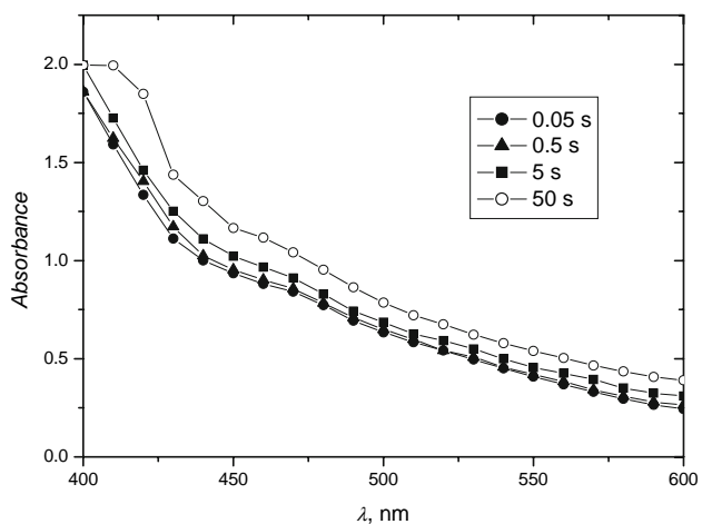
Fig. 4 Rapid scan time course of the solid \text{Fe} – \text{IAA} complex redissolved in absolute ethanol–water solvent (50:50v/v)
