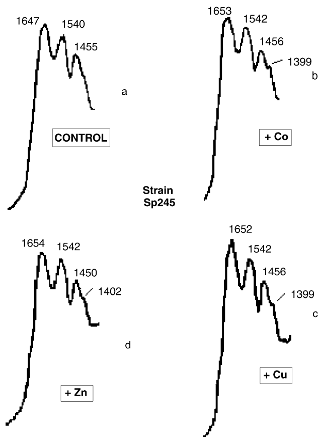
Fig. 2. Fourier transform infrared spectra of whole cells of A. brasilense Sp245 (facultative endophyte) grown (a) in the MSM (control) and in the medium with 0.2 mmol/l \text{Co}^{2+} (b), \text{Cu}^{2+} (c) or \text{Zn}^{2+} (d).
