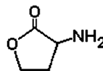
homoserine lactone
