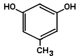
5-methylresorcinol (orcinol)
