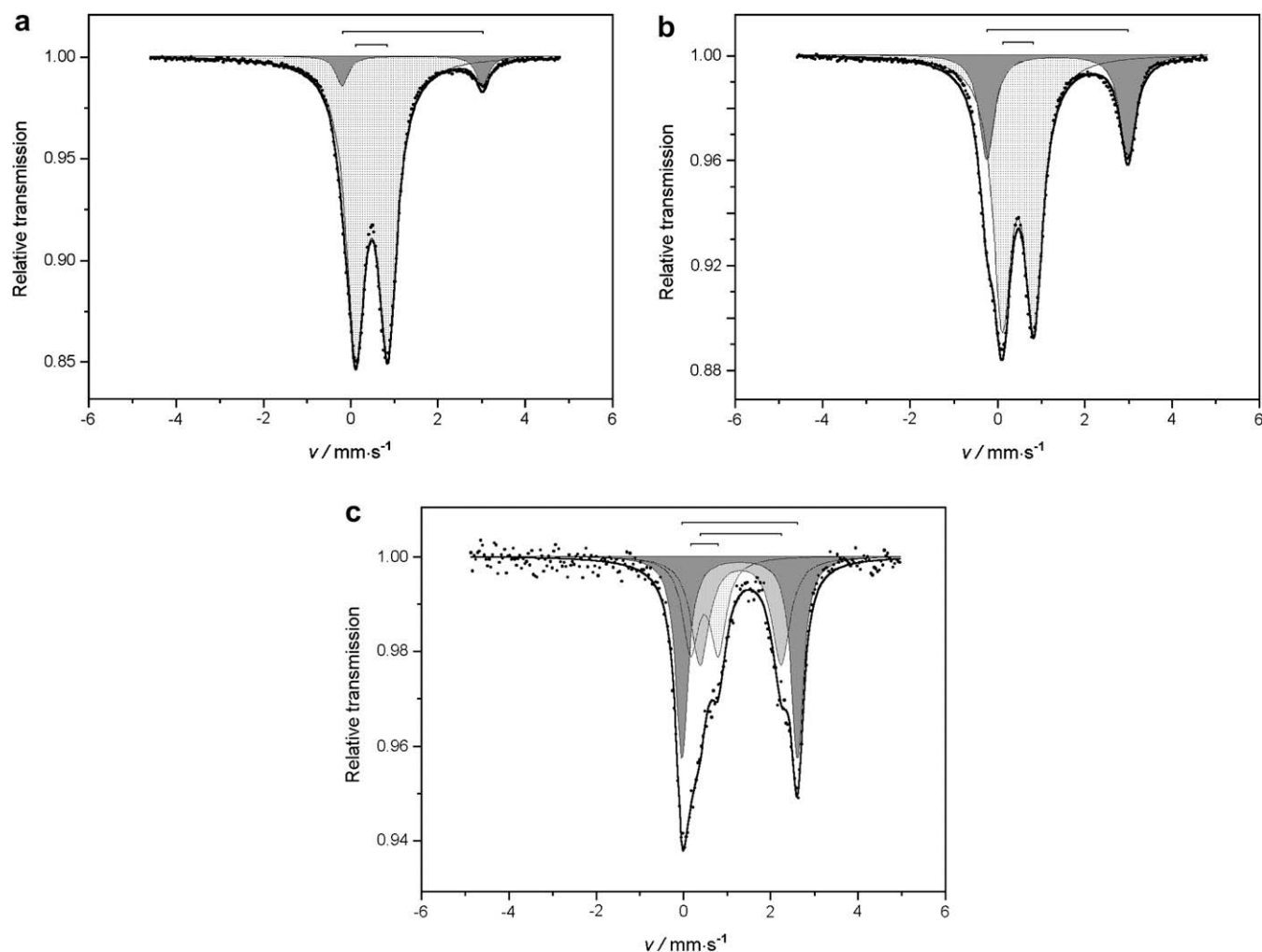
Fig. 2. Mössbauer spectra of ^{57}\text{Fe}(\text{III}) -containing aqueous solutions of 5-methylresorcinol (orcinol) rapidly frozen (a) 10 min and (b) 5.5 h after mixing, as well as of (c) the solid residue obtained by air-drying the solution at room temperature (all spectra measured at T = 80\text{ K} ). The shaded areas (quadrupole doublets) represent contributions of \text{Fe}^{\text{III}} (the most lightly shaded area) or \text{Fe}^{\text{II}} (darker shaded areas) to the whole spectrum area (defined by the outer solid-line envelope); in spectrum (c), the two more dark-shaded areas correspond to two different iron(II) species (forms 1 and 2, respectively; see Table 1). The position of each quadrupole doublet is shown by a square bracket above the spectra (the same for Figs. 3 and 4).
