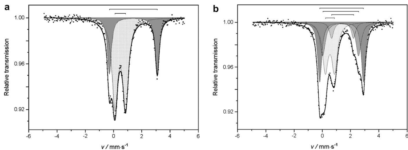
Fig. 3. Mössbauer spectra (a) of 57 Fe(III)-containing aqueous solution of 4- n -hexylresorcinol rapidly frozen 5 min after mixing and (b) of the solid residue obtained by air-drying the solution at room temperature (both spectra measured at T = 80 K). The shaded areas (quadrupole doublets) represent contributions of Fe III (the most lightly shaded area) or Fe II (darker shaded areas) to the whole spectrum area (defined by the outer solid-line envelope); in spectrum (b), the three more dark-shaded areas correspond to three different iron(II) species (forms 1–3, respectively; see Table 1).
