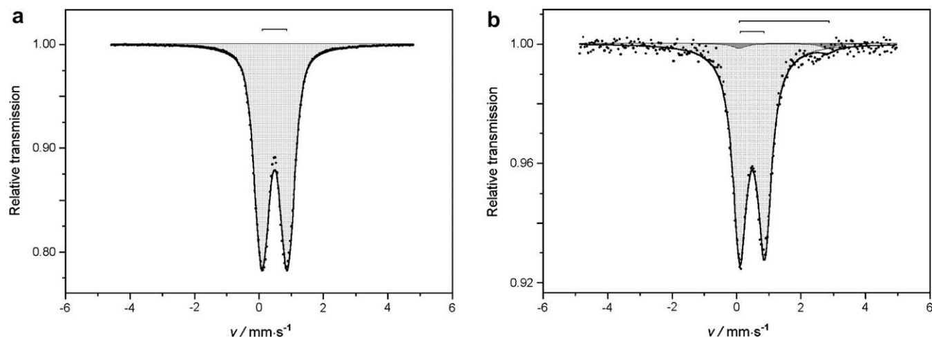
Fig. 4. Mössbauer spectra (a) of ^{57}\text{Fe}(\text{III}) -containing aqueous solution of homoserine lactone rapidly frozen 10 min after mixing and (b) of the solid residue obtained by air-drying the solution at room temperature (both spectra measured at T = 80\text{ K} ). In spectrum (b), the dark-shaded area (weak doublet with a larger quadrupole splitting) corresponds to iron(II) species (see Table 1).
