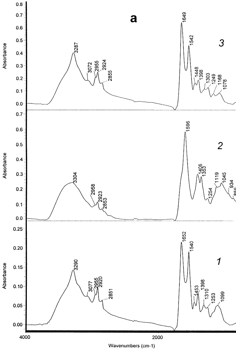
Fig. 1. FTIR-ATR spectra (a) of protein A: (1) pure ( 100\ \mu\text{g} of protein), (2) conjugated with colloidal gold ( 20\ \mu\text{g} of protein), (3) the same as 2 after interaction with human IgG, and (b) of pure human IgG.
