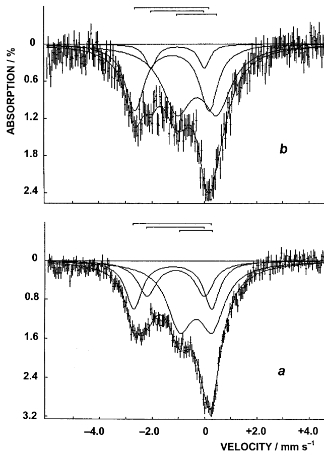
Fig. 1 Emission Mössbauer spectra of Azospirillum brasilense Sp245 living cells frozen (a) 2 min and (b) 1 h after incubation with trace 57 CoCl 2 (dried; T=80 K)
