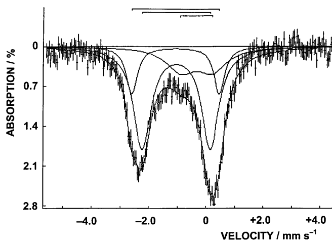
Fig. 2 Emission Mössbauer spectrum of cation-free glutamine synthetase from Azospirillum brasilense Sp245 activated by ^{57}\text{Co}^{2+} (frozen solution; T=80\text{ K} )
