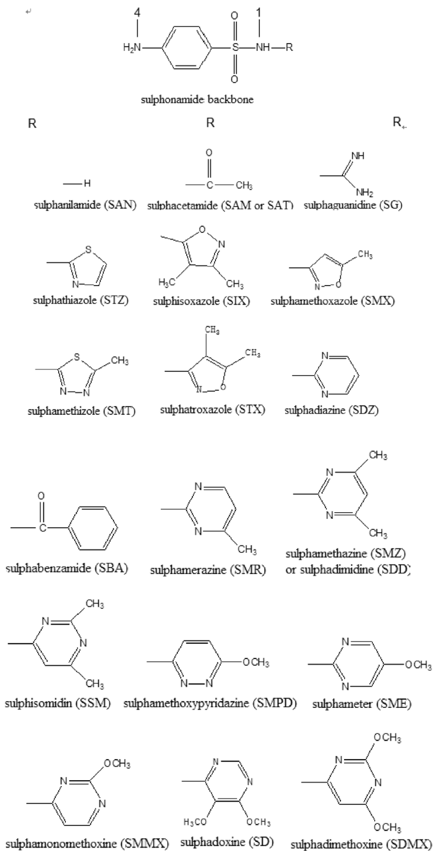
Figure 1. Structures of sulphonamides.
