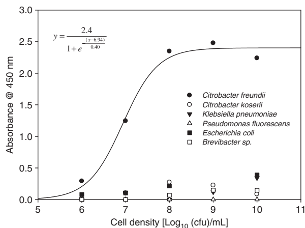
Figure 1. Sensitivity and specificity of purified anti-3C IgG measured by sandwich ELISA. IgG was diluted to 2 µg of protein per milliliter.
