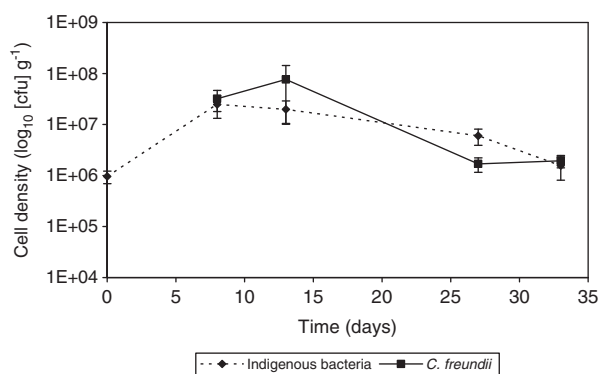
Figure 5. Monitoring the survival of C. freundii (3C) against indigenous bacteria in non-sterile sandy loam soil (pH 5.36, organic matter 5.1%, sand 60%, silt 26%, clay 14%; Camden, New South Wales, Australia) for five weeks after inoculation with 3C. Each pot was infiltrated with inoculant strain (5 mL of 10 8 cfu/mL) and kept in the greenhouse. Error bars represent 95% confidence levels ( n \geq 2 ).
