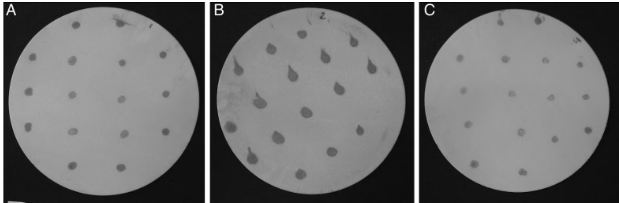
Figure 2. Comparison of the effect on colour development of immunoblots with different anti-3C IgG incubation times (0.5, 1 and 2 h). Colonies of C. freundii were prepared by direct inoculation of agar plates.
