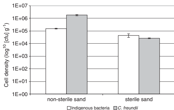
Figure 3. Survival of C. freundii in wheat seedling rhizospheres in sterile and non-sterile sand 6 weeks after inoculation measured by the optimised CIB procedure. In case of trials with sterile sand indigenous bacteria mainly introduced during plant growth. Error bars represent 95% confidence levels ( n = 3 ).
