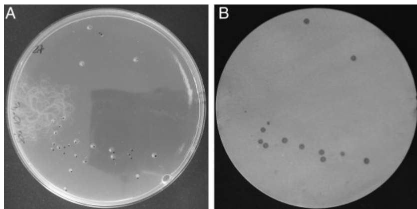
Figure 4. Modified NA spread plate and immunoblot of C. freundii recovered 4 weeks after inoculation into non-sterile sandy loam soil (pH 5.36, organic matter 5.1%, sand 60%, silt 26%, clay 14%) from Camden, New South Wales, Australia).
