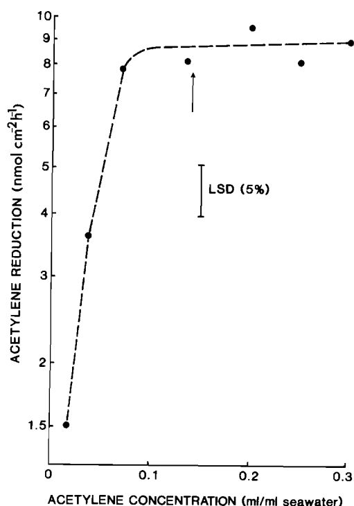
Fig. 4. Effect of acetylene concentration in seawater on acetylene reduction, measured on branching Acropora sp. rubble at Site 3 in February 1983. Arrow shows acetylene concentration used by Burris (1976)
