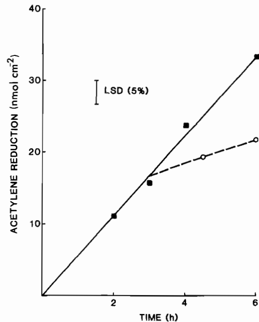
Fig. 2. Time-dependence and effect of darkness on acetylene reduction, measured on limestone substrata sampled randomly at Site 3, December 1981. Continuous line: samples left in light; dashed line: samples darkened at 3 h. LSD: least-significant difference
