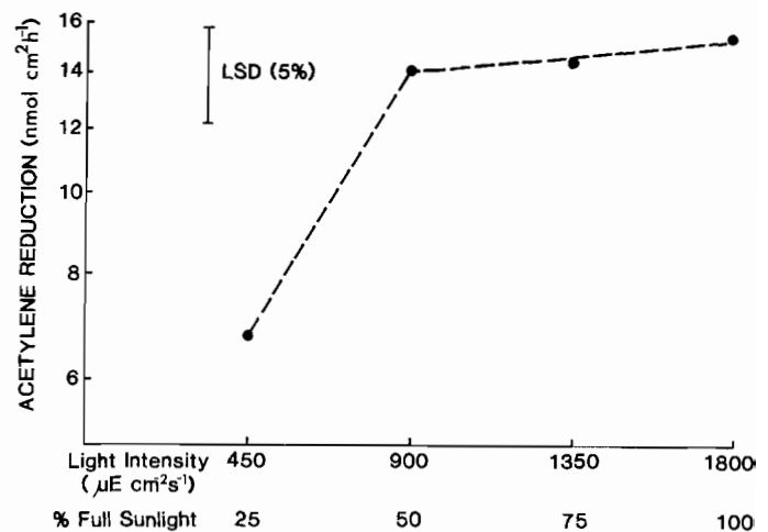
Fig. 3. Effect of light saturation on acetylene reduction, measured on limestone substratum collected randomly at Site 3 in February 1983
