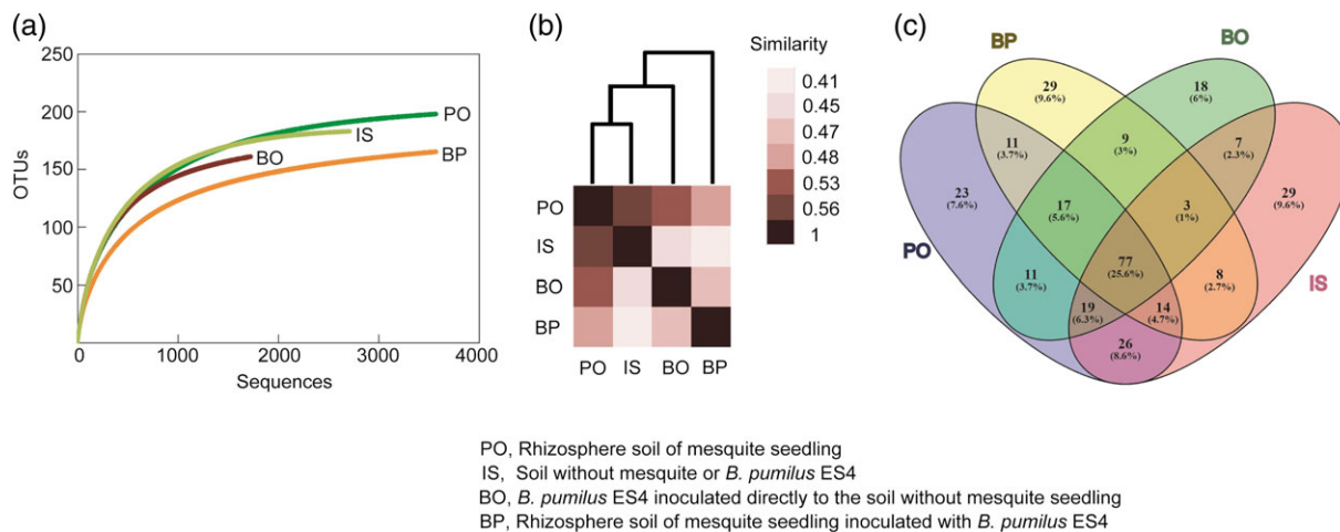
FIGURE 3 (a) Rarefaction curves, (b) cluster analysis, and (c) Venn diagram of soil bacterial communities with 301 operational taxonomic units (OTUs) defined at 97% similarity. Rarefaction curves were calculated by 100 randomizations without extrapolation in EstimateS 9.1.0. Asymptotic curves indicate that sequencing depth adequately represents the estimated richness. Cluster analysis by Jaccard's index shows the similarity in the composition of OTUs among samples. Venn diagram was constructed with Venny 1.0 ( http://bioinfo.gp.cnb.csic.es/tools/venny/index.html ) and represents the number of OTUs, unique and shared (overlapping areas) between combinations of samples. Integer values or percentages in parenthesis accumulate 301 OTUs (100%) analyzed [Colour figure can be viewed at wileyonlinelibrary.com ]
