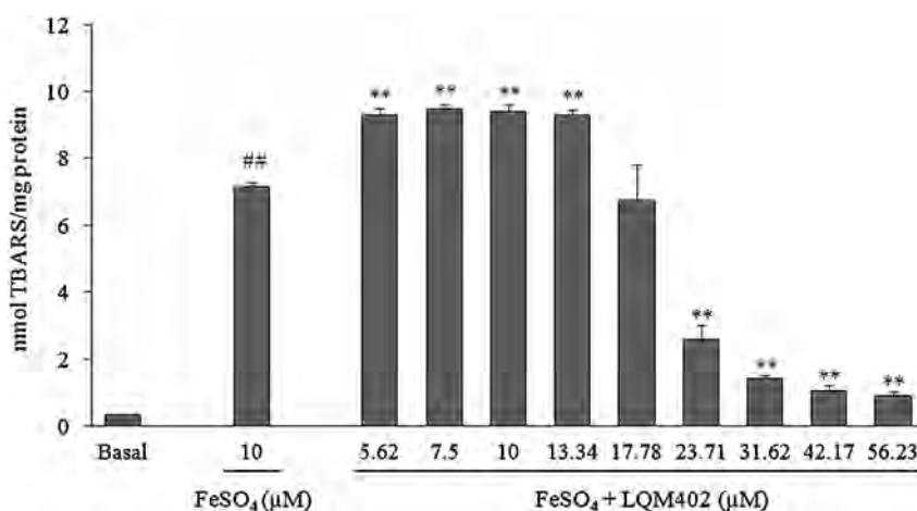
Fig. 9. LQM402 enhances and inhibits \text{FeSO}_4 -induced TBARS production. Lipid peroxidation was induced in rat brain homogenate by 10 \mu\text{M} \text{FeSO}_4 alone or simultaneously adding LQM402 at different concentrations (5.62–56.23 \mu\text{M} ). TBARS production was measured at 540 nm. TBARS induced by \text{FeSO}_4 was enhanced with 5.62–13.34 \mu\text{M} LQM402 and was inhibited in a concentration-dependent manner at concentrations of 23.71 \mu\text{M} and higher. The graph shows the mean and standard errors of three independent experiments. ## p < 0.01 indicates significant difference of LQM402-treated groups compared to the basal level and ** p < 0.01 represents significant differences compared with \text{FeSO}_4 .
