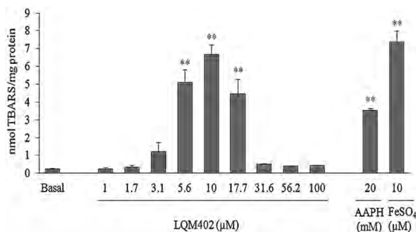
Fig. 8. LQM402 is an inducer of lipid peroxidation. Rat brain homogenate (2 mg/ml protein) was incubated with LQM402 at several concentrations (1–100 \mu\text{M} ) at 37 °C for 3 h. TBARS production was measured at 540 nm. Significant TBARS production, indicated by p < 0.01 , was only observed at concentrations from 5.62 \mu\text{M} to 17.78 \mu\text{M} . At 10 \mu\text{M} , LQM402 is a more potent lipid peroxidation inducer than AAPH (20 mM) and is similar to \text{FeSO}_4 (10 \mu\text{M} ). The graph shows the means and standard errors of three independent experiments.
