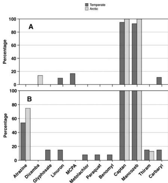
Fig. 1. Susceptibility of Rhizobium leguminosarum bv. viciae (A) and Mesorhizobium spp. (B) strains from temperate and arctic origin to different pesticides when applied at 450 \mu\text{g} per disk. A total of 25 R. leguminosarum bv. viciae (18 temperate, 7 arctic) and 15 Mesorhizobium sp. (7 temperate, 8 arctic) strains were tested.
