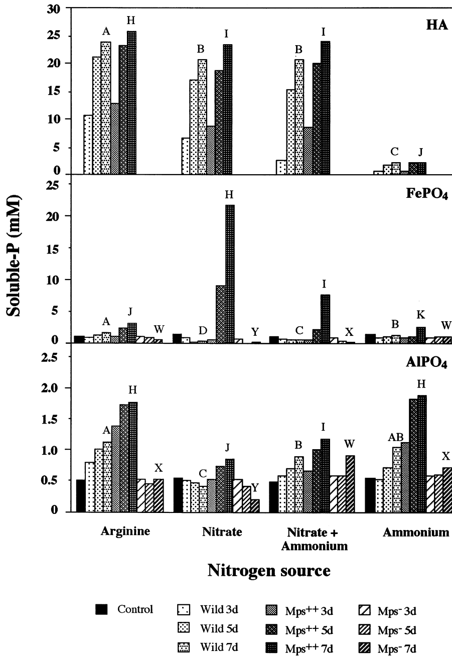
Fig. 1. Solubilization of HA, FePO 4 and AlPO 4 by P. rugulosum isolate IR-94MF1 and its Mps ++ and Mps - mutants in liquid medium using sucrose as the C source and different N sources (3.7 mM arginine, 18 mM nitrate, 18 mM nitrate+ammonium and 0.7 mM ammonium) after 3 (3d), 5 (5d) and 7 (7d) days of incubation. Values are means of three replicates. Means labeled with the same letter are not significantly ( P > 0.01 ) different according to the LSD test used with the rank procedure.
