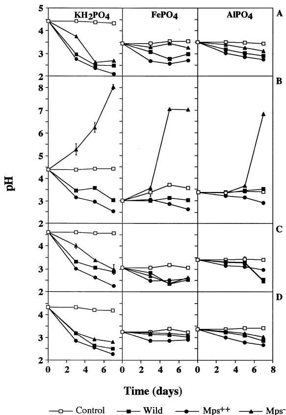
Fig. 2. Changes of the pH of the culture filtrate of P. rugulosum IR-94MF1 and its Mps^{++} and Mps^- mutants cultivated in liquid media containing sucrose as the sole C source and different N or P sources: (A) 3.7 mM arginine; (B) 18 mM nitrate; (C) 18 mM nitrate+ammonium; and (D) 0.7 mM ammonium. Values are means of three replicates. Error bars ( \pm S.D.) are shown when larger than the symbol.
