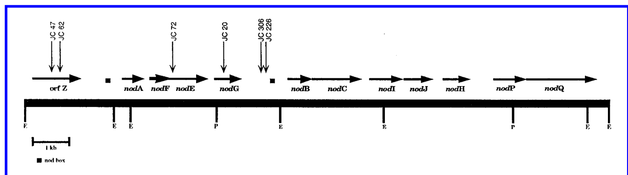
Fig. 1. Physical and genetic map of open reading frame orfZ and nodAFEG genes of Rhizobium sp. strain N33. Vertical arrows indicate position of various Tn5 insertions in orfZ and in the nodAFEG genes. The nod box and positions and direction of transcription of orfZ and nodAFEGBCIJHPQ are indicated. Restriction sites for mapping are indicated: E, EcoRI ; P, PstI .
