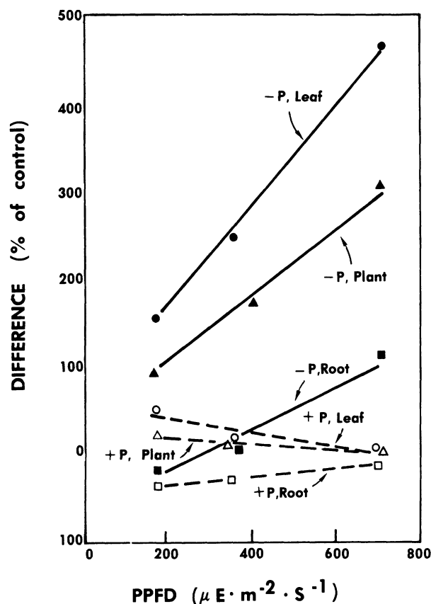
FIG. 1. Per cent change with PPFD in VAM plant parameters relative to non-VAM plants treated with additional P (+P control) or not treated (-P control). Per cent difference was calculated as [(VAM \text{ plant} - \text{control}) / \text{control}] \times 100 . The VAM plants were colonized by the fungus Glomus fasciculatum .
