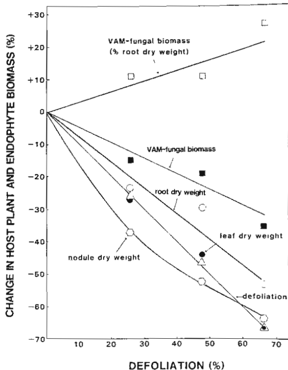
Fig. 2. Changes in host-plant and endophyte biomass as a function of defoliation. Values represent changes relative to those of the undefoliated controls. Absolute values of controls: see tables.
