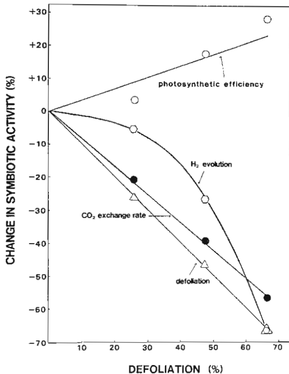
Fig. 1. Changes in symbiotic activity (photosynthesis, H 2 evolution) as a function of defoliation. Values represent changes relative to those of the undefoliated controls. Absolute values of controls: see tables.
