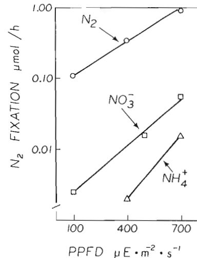
Figure 4. Nitrogen fixation in pea plants grown at different photosynthetic photon flux densities (PPFD) with NO 3 - or NH 4 + or without combined-N (N 2 ). N 2 fixation values were computed from C 2 H 2 -dependent C 2 H 4 and H 2 evolution data by the formula:
