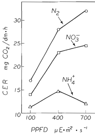
Figure 2. CO 2 -exchange rates (CER) in pea plants grown at different photosynthetic photon flux densities (PPFD) with NO 3 - or NH 4 + or without combined-N (N 2 ). The fifth leaf in each plant was used in these measurements.
