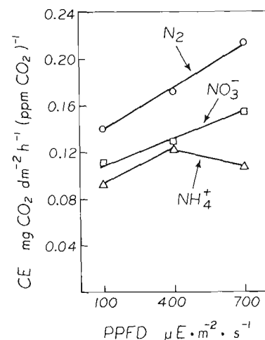
Figure 1. Carboxylation efficiency (CE) in pea plants grown at different photosynthetic photon flux densities (PPFD) with \text{NO}_3^- or \text{NH}_4^+ or without combined-N ( \text{N}_2 ). Each datum represents the slope (at the \text{CO}_2 -compensation point) of a regression line through data points determined by four internal \text{CO}_2 concentrations and the corresponding \text{CO}_2 -exchange rates. The fifth leaf in each plant was used in these measurements.
