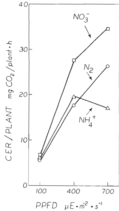
Figure 3. CO 2 -exchange rates (CER) in pea plants grown at different photosynthetic photon flux densities (PPFD) with NO 3 - and NH 4 + or without combined-N (N 2 ). CER was determined in the entire plant by sequential insertion of plant segments into the assay chamber, and summing the data from all segments.
