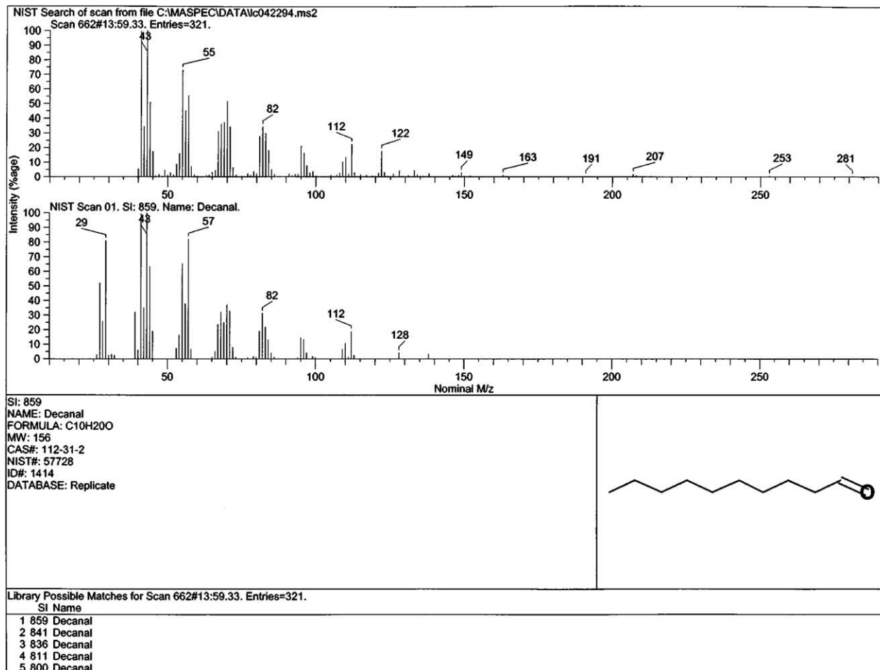
Fig. 4. GC–MS data analysis of n -decanal. The GC–MS analysis and the subsequent database search yielded 23 organic volatile compounds. Compounds, with similarity index (SI) > 850 from the database search, were considered for the in vitro antifungal assays in divided plates.
