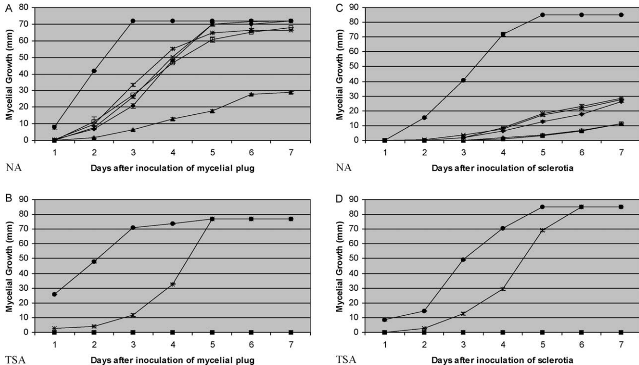
Fig. 3. Bacterial antifungal-volatile assays (sealed plates). (A) Mycelial inhibition on NA/PDA. (B) Mycelial inhibition on TSA/PDA. (C) Sclerotial inhibition on NA/PDA. (D) Sclerotial inhibition on TSA/PDA. Of the five isolates presented in the figure, isolates, PA-23 (X's), DF190 (filled diamond), DF200 (square), DF209 (filled triangle) had 100% inhibition of the mycelial plug (Fisher's LSD=0.58 mm) and the sclerotia (Fisher's LSD=0.66 mm) on TSA, as compared to the control (filled circle). Bacterial treatments had significantly higher inhibition of the sclerotial germination (Fisher's LSD=1.53 mm) than the mycelial growth (Fisher's LSD=2.22 mm) on NA plates. Isolates PA-23, DF190, DF200 and DF209 are seen at the bottom (0 mm) of (B and D), due to their 100% inhibition of both mycelial and sclerotial germination on TSA. Values used are the mean of the radial mycelial growth of S. sclerotiorum . Each treatment had four replicates and the experiments were done twice. Bars represent the standard error of mean of eight replicates.
