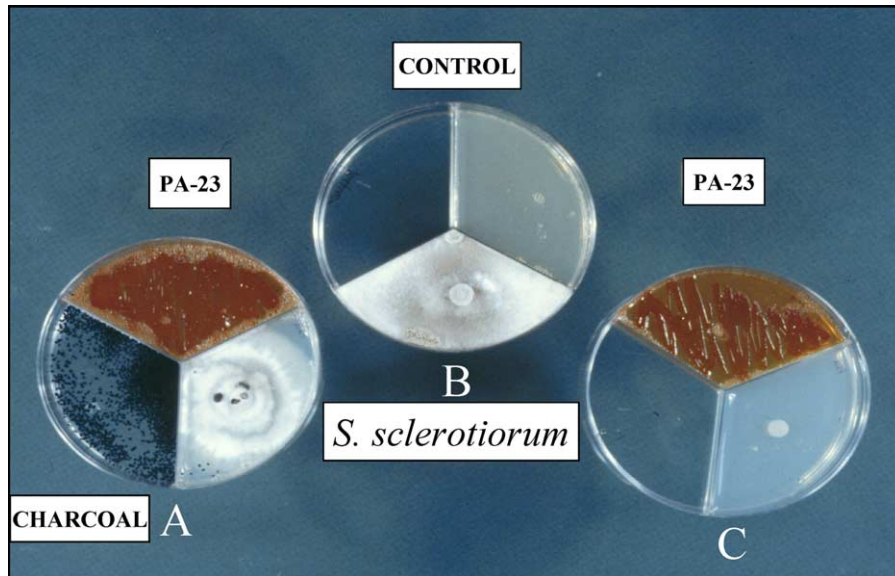
Fig. 1. Bacterial antifungal-volatile activity in divided plates. Mycelial plug growth was completely inhibited in the presence of the bacteria streaked in a different compartment (C), as compared to the control (B), which had no bacteria. Mycelial growth was unaffected by the presence of volatile producing bacteria, when the third compartment of the plates was amended with activated charcoal (A). Charcoal adsorbs volatiles as soon as they are produced, and hence no inhibitory effect was observed.
