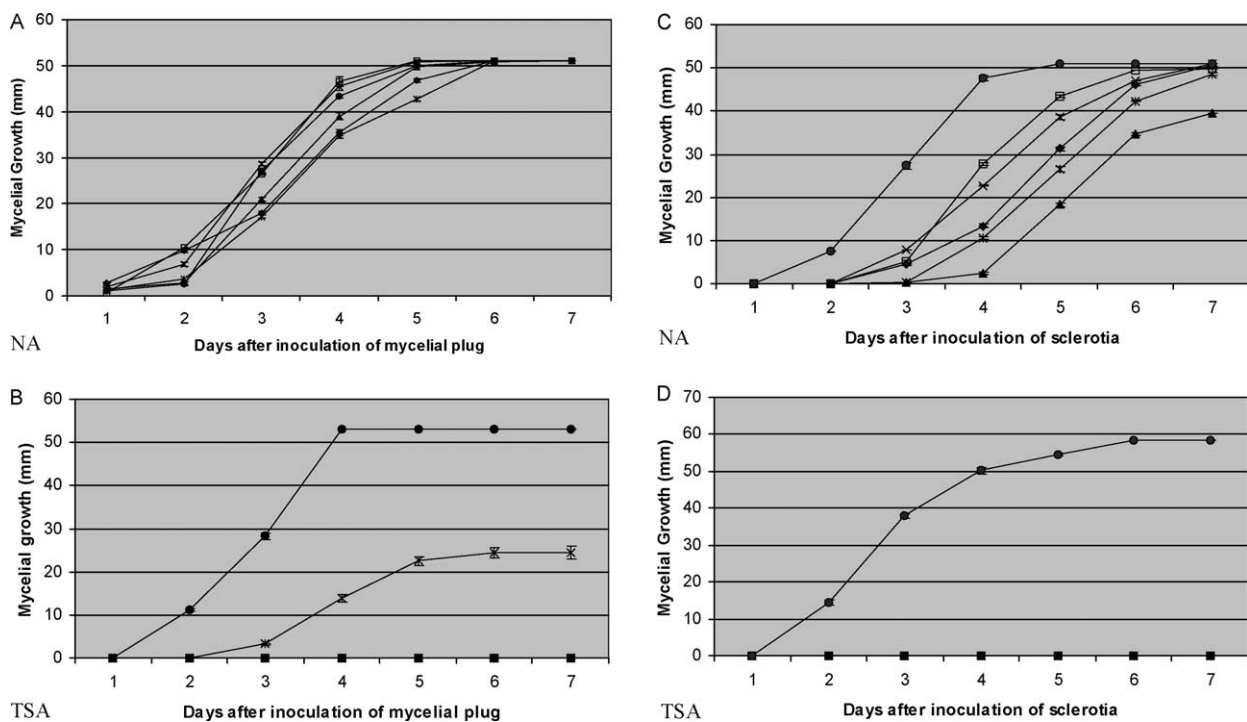
Fig. 2. Bacterial antifungal-volatile assays (divided plates). (A) Mycelial inhibition on NA/PDA. (B) Mycelial inhibition on TSA/PDA. (C) Sclerotial inhibition on NA/PDA. (D) Sclerotial inhibition on TSA/PDA. Bacterial volatile production was enhanced by TSA (B and D), resulting in higher inhibition of mycelial growth and sclerotial germination on TSA than on NA (A and C). Also, in the NA plates, the inhibition of the sclerotial germination was higher than the mycelial inhibition. In the NA plates, mycelial growth in bacterial treatments were significantly different from the control up to 5 days post-inoculation of the mycelial plug (Fisher's LSD = 1.06 mm) and up to 6 days post-inoculation of sclerotia (Fisher's LSD = 0.78 mm). Of the five isolates presented in the figure, isolates, PA-23 (X's), DF190 (filled diamond), DF200 (square), DF209 (Filled triangle) had 100% inhibition of the mycelial plug (Fisher's LSD = 1.08 mm) and the sclerotia (Fisher's LSD = 0.56 mm) on TSA, as compared to the control (filled circle). Isolates PA-23, DF190, DF200 and DF209 are seen at the bottom of the graph (0 mm) in (B), due to their 100% inhibition of the mycelial growth on TSA. Isolate DF35 (asterisk) showed 50% inhibition of mycelial growth and 100% inhibition of sclerotial germination in TSA divided plates. All the bacterial treatments are seen at the bottom of the graph (0 mm) in (D), due to their 100% inhibition of sclerotial germination on TSA. The values used are the mean of the radial mycelial growth of S. sclerotiorum . Each treatment had four replicates and the experiments were done twice. Bars represent the standard error of mean of eight replicates.
