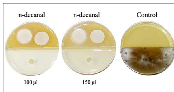
Fig. 5. Antifungal activity of n -decanal in divided plates. The compounds, identified through GC–MS analysis, used in this assay are synthetic chemicals that were purchased. Each of the compounds was tested for antifungal activity by placing 100 and 150 µl of each compound, singly and in combination with tryptic soy broth (TSB), on sterile filter paper discs placed on TSA in divided agar plates. TSB did not have any positive or negative effect on the antifungal activity of any of the 23 compounds tested.
