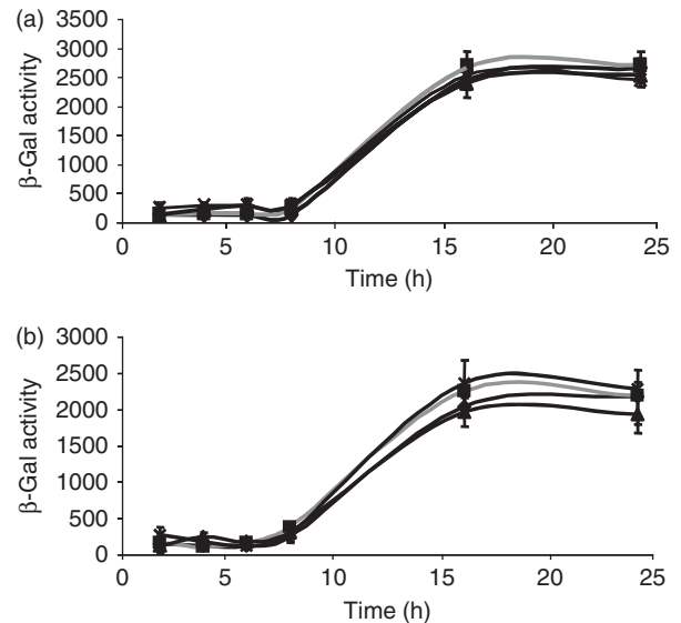
Fig. 1. Time course of prnA and phzA expression in Pseudomonas chlororaphis PA23 (◆, wild type), PA23-63 (■, PHZ - ), PA23-8 (▲, PRN - ) and PA23-63-1 (×, PHZ - PRN - ). Cultures containing a prnA-lacZ fusion (a) or a phzA-lacZ fusion (b) were analyzed for \beta -galactosidase activity throughout growth as described in Materials and methods. Note: for some data points, error bars representing SD are too small to be shown on the graph.
