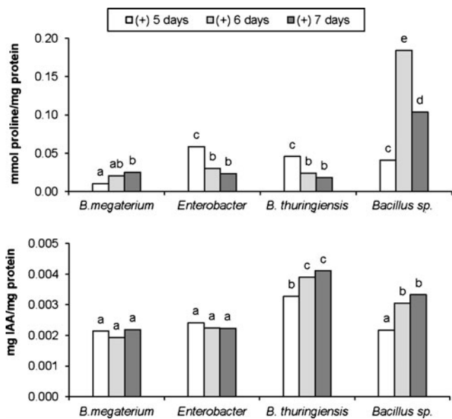
Fig. 4 Cell proline accumulation and indoleacetic acid (IAA) production by native and reference bacteria growing in axenic nutrient medium supplemented with PEG (15 %) at different time intervals (from 5 to 7 days)
