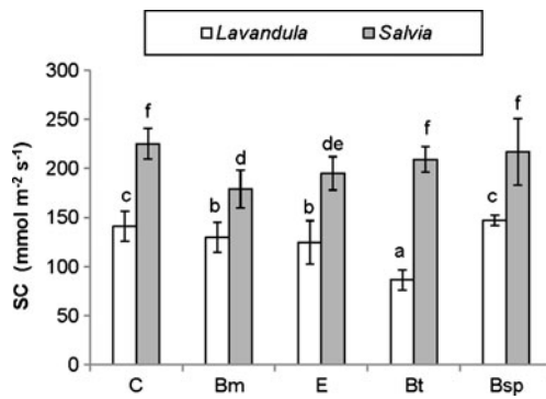
Fig. 1 Effect of autochthonous bacterial strains Enterobacter sp. ( E ), B. thuringiensis ( Bt ) and Bacillus sp. ( Bsp ) and the reference B. megaterium ( Bm ) on stomatal conductance ( SC ) in two autochthonous plants ( L. dentata and S. officinalis ) growing in a natural arid Mediterranean soil under drought conditions. Means followed by the same letter are not significantly different ( P \leq 0.05 ) after ANOVA and Duncan tests
