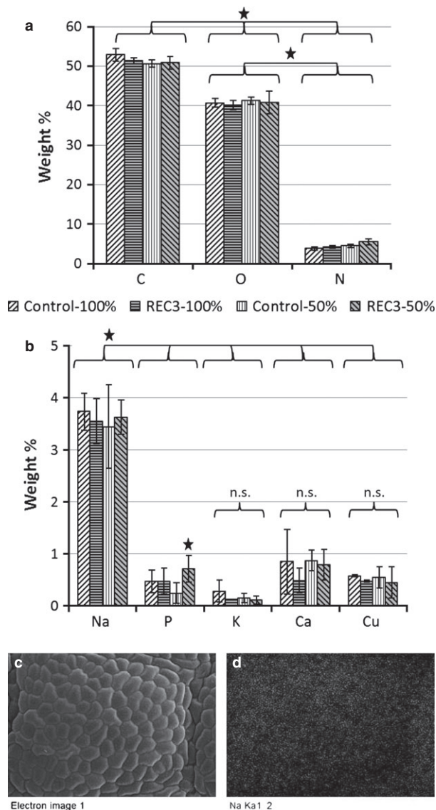
Fig. 2. SEM-EDS microanalysis of leaf mineral composition of Azospirillum -inoculated and not inoculated control strawberry plants grown in 50% or 100% Hoagland solution (average of three replicates). a: Organic fraction represented by C, O and N. b: mineral fraction represented by Na, P, K, Ca and Cu. (*, P < 0.05 ; n.s., not significant). c: Scanning micrograph of analysed leaf area (1000 \times magnification). d: EDS map of the relative distribution of Na in strawberry leaves of inoculated plants grown in 50% Hoagland solution.
