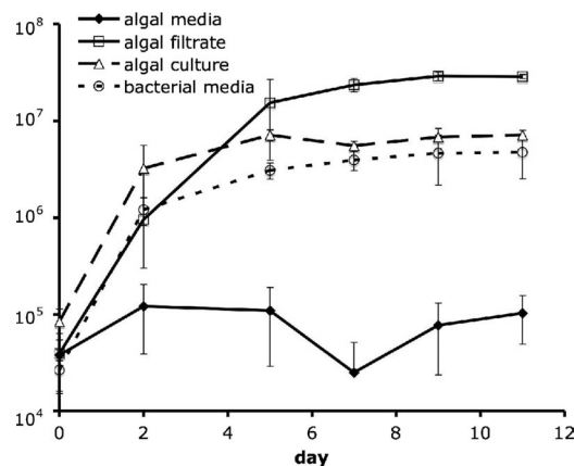
FIG. 2. Abundance of RCA cluster strain LE17 over time in seawater with inorganic nutrient ( f/4 algal medium), in L. polyedrum stationary culture filtrate, in log-phase L. polyedrum whole culture, and in 100 \times -diluted ZoBell bacterial medium (seawater with 0.05 g peptone and 5 mg yeast extract \text{liter}^{-1} ) measured with flow cytometry. Error bars represent standard deviations of triplicate incubations.
