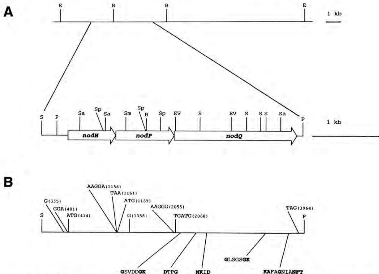
Fig. 2. A , Physical and genetic map of the nodHPQ region. Restriction sites are marked: EcoRI (E), BamHI (B), SacI (Sa), SphI (Sp), SmaI (Sm), EcoRV (EV). B , Horizontal line represents Rhizobium tropici strain CFN299 nodHPQ zone, depicted in A . Extreme SacI (S) and PstI (P) restriction sites are indicated. Above horizontal line: translation signal sequences (see Results) followed by their respective positioning as submitted to GenBank. Numbers refer to first letter of corresponding sequences, except for position 2068, which indicates the 'A' in the overlap of the nodP stop-codon and the nodQ start-codon. The two guanines are the nucleotides that are different from the R. tropici strain CIAT899 nodHPQ region. Under the horizontal line: amino acid sequences of the GTP-, ATP-, and PAPS (3'-phosphoadenosine 5'-phosphosulfate)-binding motifs. Conserved amino acid residues shown in bold (see Results).
