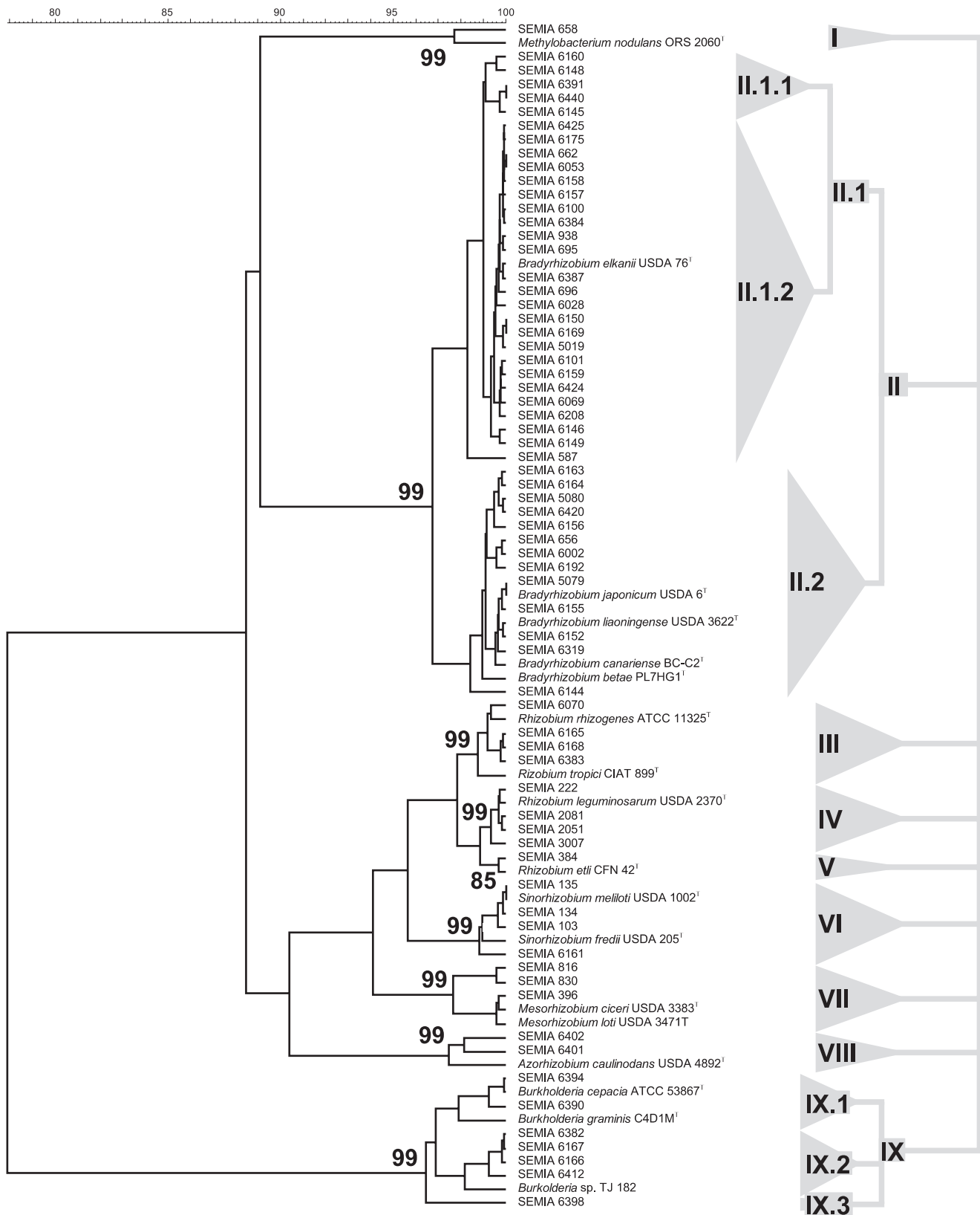
Fig. 1. Phylogenetic tree based on the 16S rRNA sequences of 68 strains, N 2 -fixing symbionts isolated from 46 legumes and officially recommended for the use in Brazilian commercial inoculants. GeneBank accession numbers of SEMIA strains (Table 2) and of type strains (material and methods) are given in the text. Phylogenetic trees were generated using MEGA version 3.1 with default parameters, K2P distance model and the Neighbor-Joining algorithm.
