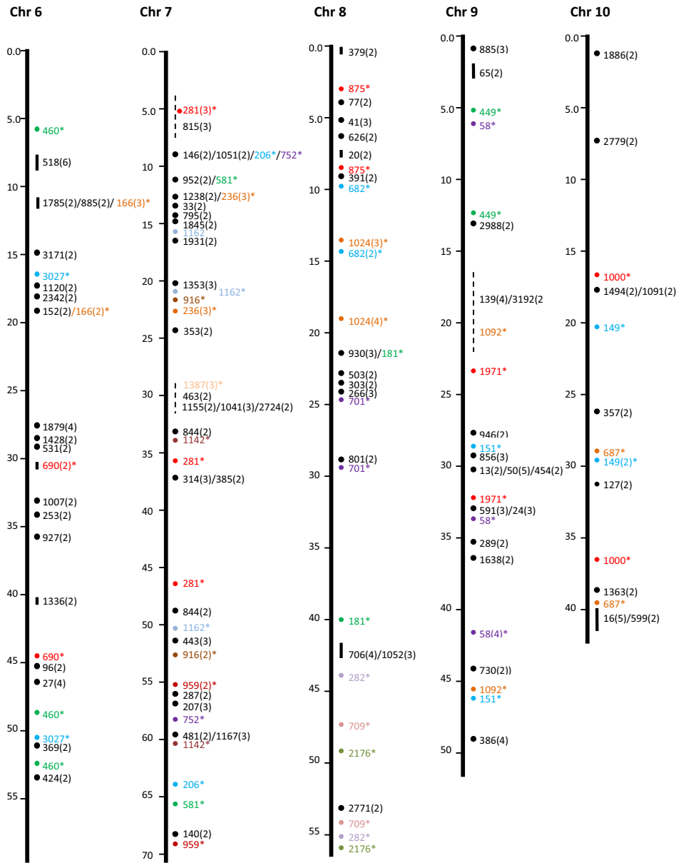
Figure 2 Identification of microsynteny through comparative sequence analysis (chr 6 through chr 10). tBLASTX searches were conducted using BAC contig-associated BAC end sequences as queries against the zebrafish genome sequence. The putative conserved microsynteny are presented along the 25 zebrafish chromosomes (chr 1 through chr 25). The position of the zebrafish sequence is shown on the left of each chromosome bars in million base pairs. The conserved microsynteny are indicated on the right side of the chromosome bars, with the numbers representing the contig numbers of the BAC assembly of the catfish physical map [41]. Circles represent short syntenic regions and short vertical lines represent relatively longer conserved syntenic regions proportional to the length of the bar with a number in parenthesis representing the number of conserved sequences within the microsynteny. The microsynteny designated with asterisks (*) are those with duplicated conservation of the microsynteny that are color-coded to facilitate the visualization of the duplicated syntenic regions along the chromosome. Duplicated syntenic regions refer to a conserved genomic segment between the catfish genome and the zebrafish genome that is duplicated in the zebrafish genome such that identical or nearly identical significant hits are generated from two chromosomal regions of the zebrafish genome using a single catfish genome segment (say it is a contig or a scaffold) as the query. In just few cases, this term is used in an extended fashion to include those that are tripled in the zebrafish genome.
