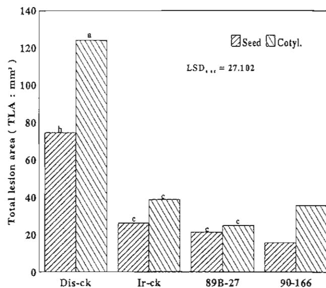
Fig. 2. Total lesion area (TLA) caused by Pseudomonas syringae pv. lachrymans on leaves challenge-inoculated by plant growth-promoting rhizobacteria (PGPR; Pseudomonas putida 89B-27 and Serratia marcescens 90-166) seed and cotyledon treatments. Seed = seed treatment with PGPR; Cotyl. = cotyledon injection with PGPR; Dis-ck is a noninduced, pathogen-inoculated control; Ir-ck is a classic induced resistance control by preinoculation of Colletotrichum orbiculare on the first leaves.
