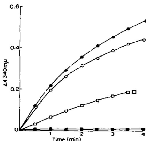
Fig. 8. The effect of cysteine and EDTA on NAD reduction by triosephosphate dehydrogenase from A. vinelandii . Each cuvette contained (in \mu\text{moles}/0.8\text{ ml} final volume): sodium pyrophosphate (pH 8.5) 18; sodium arsenate (pH 8.5) 4.2; DL-glyceraldehyde 3-phosphate, 0.38; NAD, 0.25; enzyme, 0.23 mg protein. Reaction was initiated by the addition of mixed glyceraldehyde 3-phosphate/arsenate reagent. Temperature 30^\circ . ●—●, with 0.8 \mu\text{mole} EDTA (pH 8.5); ○—○, with 3.5 \mu\text{moles} cysteine hydrochloride (pH 8.5); ■—■, with 0.25 \mu\text{mole} NADP replacing NAD and 0.8 \mu\text{mole} EDTA (pH 8.5); □—□, no additions.
