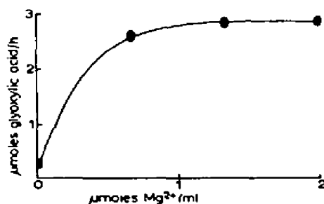
Fig. 2. Isocitrate lyase activation by Mg^{2+} . Thunberg tubes contained reagents described under Fig. 1, except: A. vinelandii extract, 0.5 mg; EDTA, 2 \mu moles; MgCl_2 , total as indicated, in final volume of 3.0 ml. Reaction was for 15 min at 30° after 5 min preincubation.
