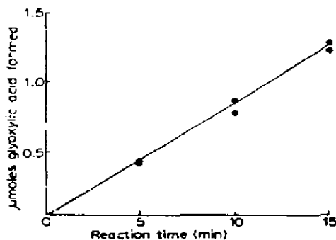
Fig. 6. Linearity of isocitrate lyase reaction with time. Warburg flasks contained (in \mu moles/3.0 ml final vol., ac): Tris buffer (pH 7.6) 200; MgCl 2 , 6; EDTA, 2; Na 2 -DL-isocitrate (side-arm), 30; plus A. vinelandii extract, 0.78 mg. Reaction was started after 30 min preincubation at 30° and stopped at the times indicated.
