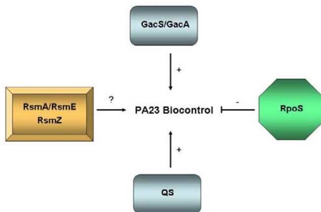
Fig. 2 Regulation of Pseudomonas chlororaphis PA23 biocontrol. In PA23, the GacS/GacA two-component signal transduction system positively regulates expression of antibiotics and degradative enzymes. The stationary phase sigma factor, RpoS, has a repressive effect on AF activity, while the PhzI/R QS system positively affects fungal inhibition. Two Rsm protein components have also been identified (RsmA and RsmE) together with a regulatory RNA ( RsmZ ). The way in which the Rsm components influence PA23 biocontrol is currently under investigation.
