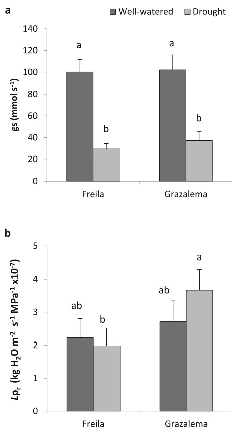
Fig. 2. Stomatal conductance ( g_s ) (a) and root hydraulic conductivity ( L_p ) (b) in Olea europaea trees from different locations, Freila with low annual precipitation, and Grazalesma with high annual precipitation. The trees were grown either under well-watered conditions or under drought stress for five weeks. Different letters above the bars indicate significant differences among treatment means after Tukey's test at p = 0.05 .
